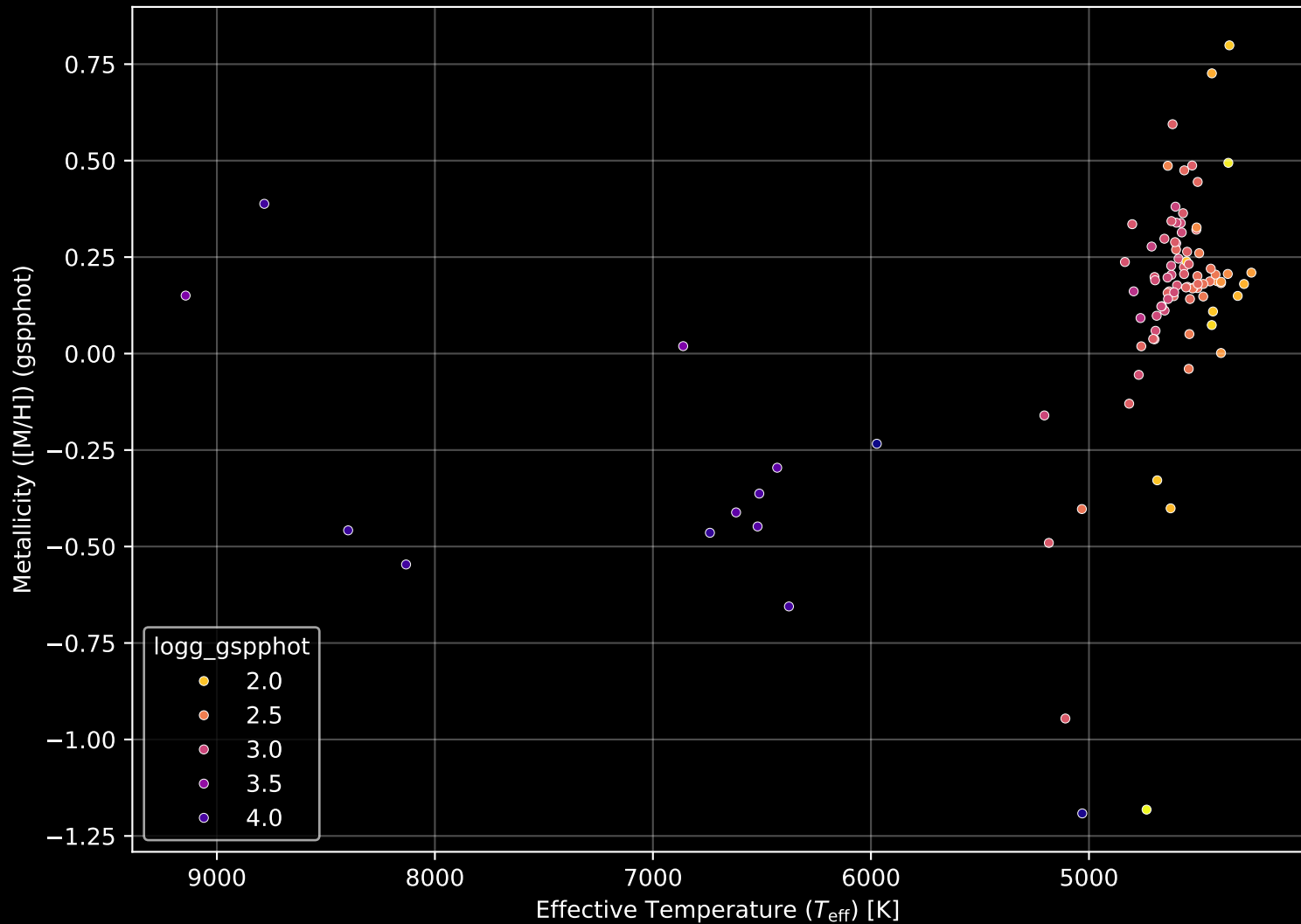
APOGEE DR17 Field: [LMC34] Stellar Population Parameters (n= 98)
