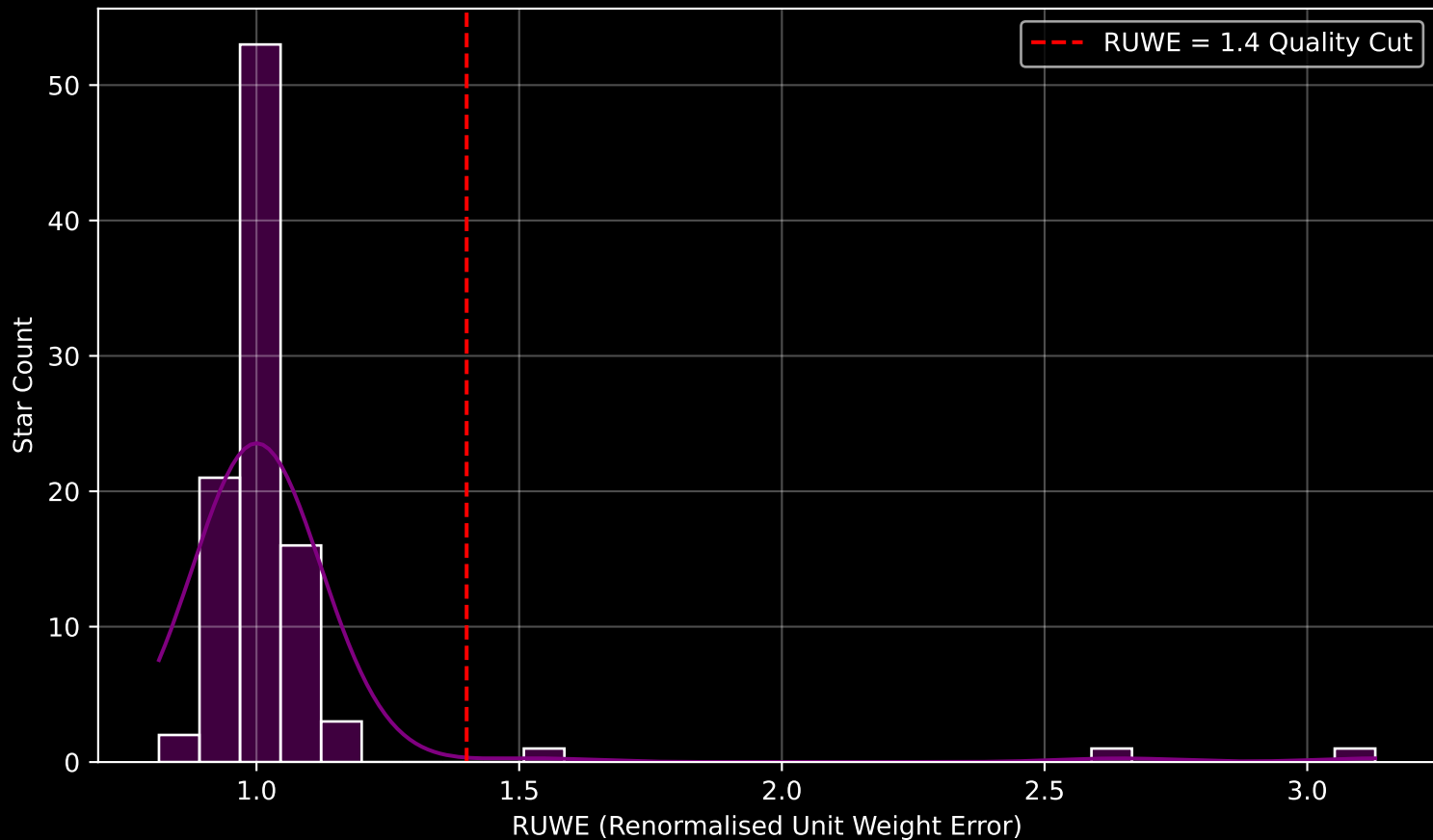
GAPOGEE DR17 Field [LMC34] RUWE Distribution (n= 98)
