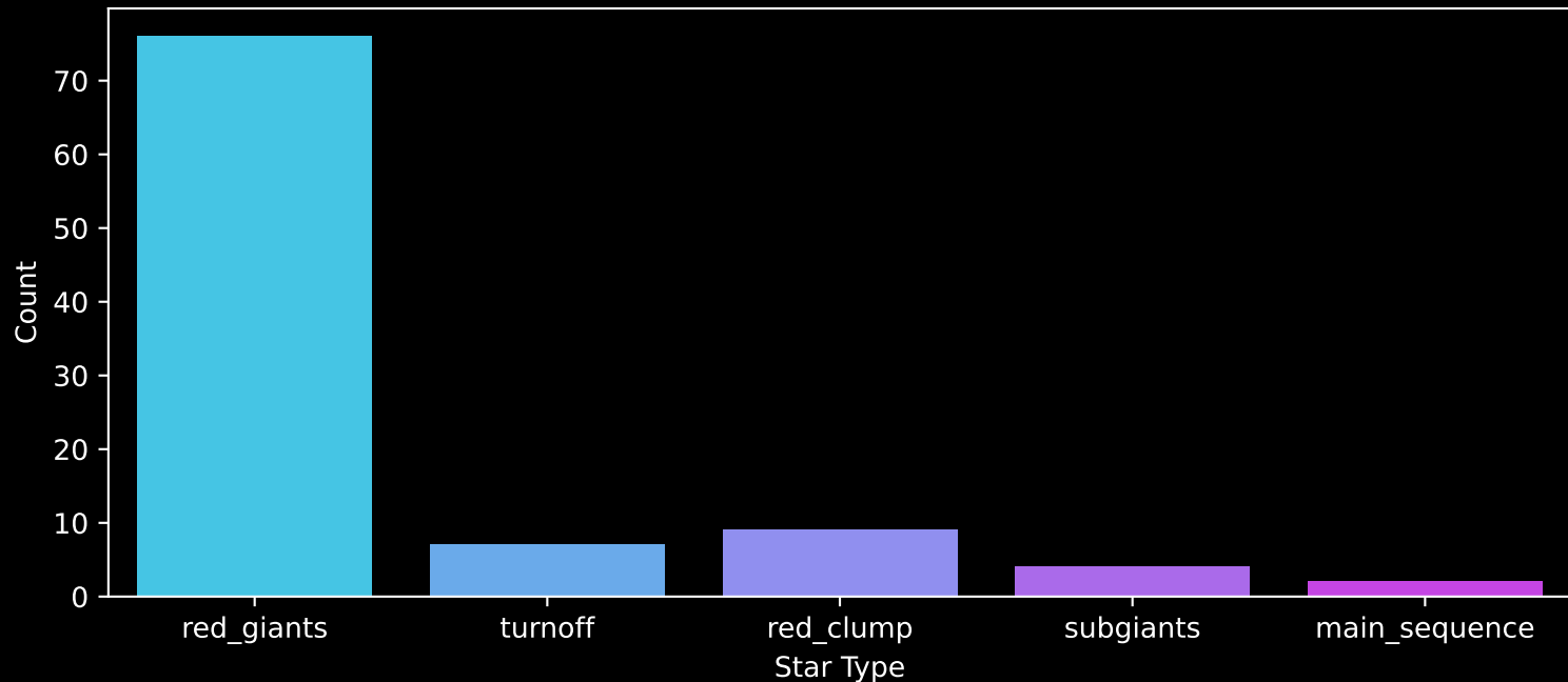
APOGEE DR17 Field: [LMC34] Count plot of Star Type
