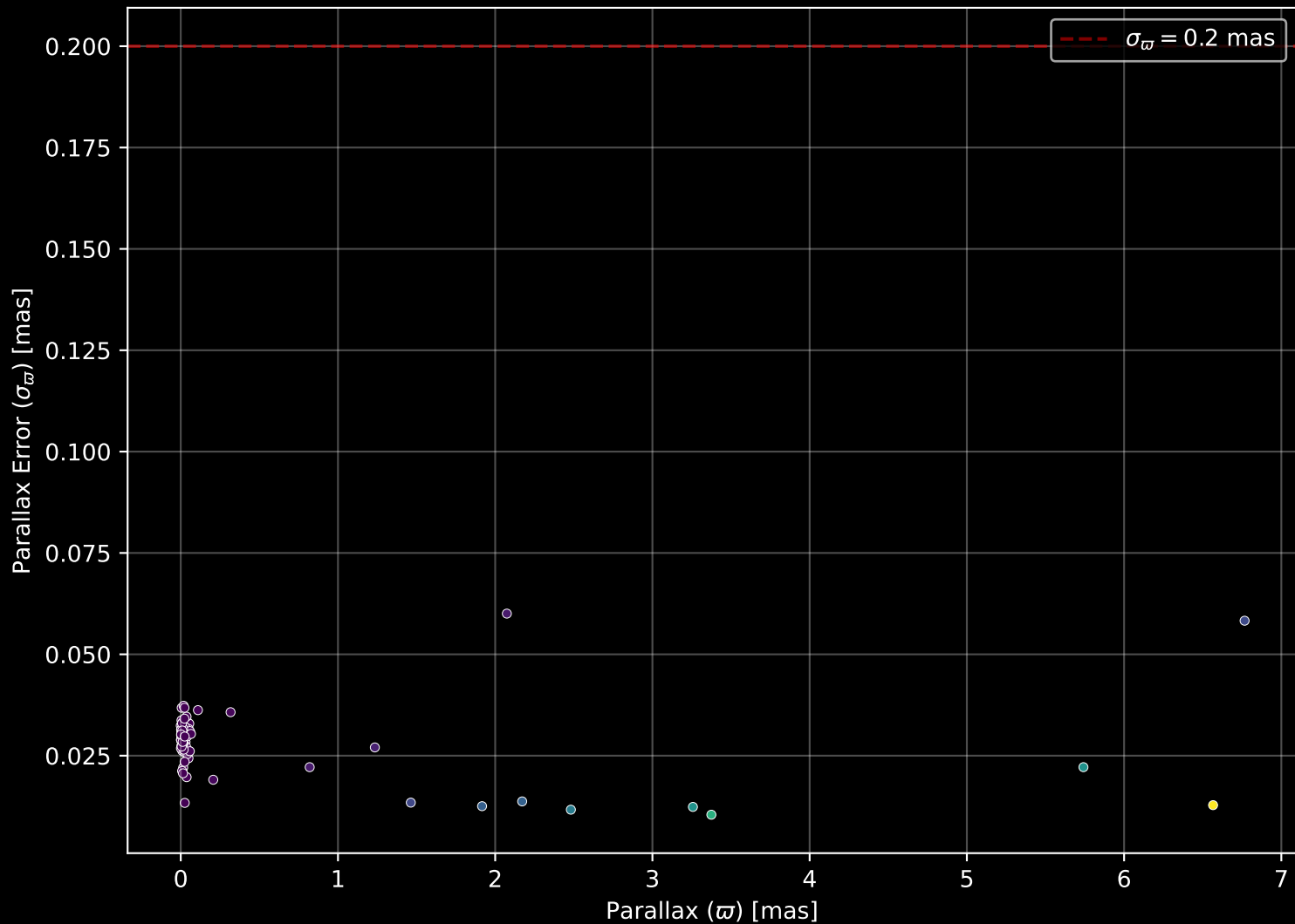
APOGEE DR17 Field: [LMC34] Parallax Quality (n= 98)
