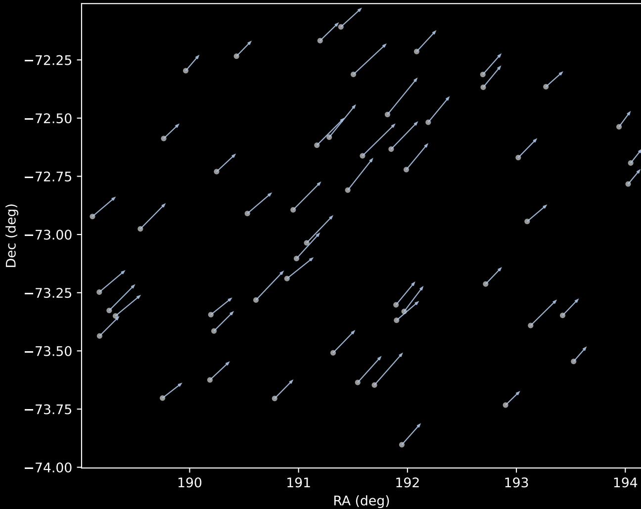
APOGEE DR17 Cluster 1 Proper Motion Vectors (n=53)
