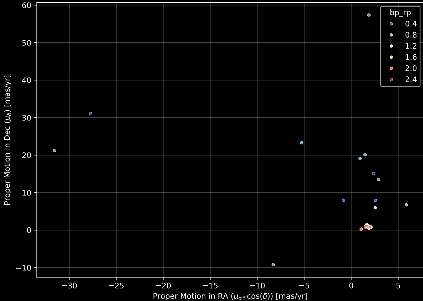
APOGEE DR17 Field: [LMC34] Proper Motion Diagram (n= 98)
