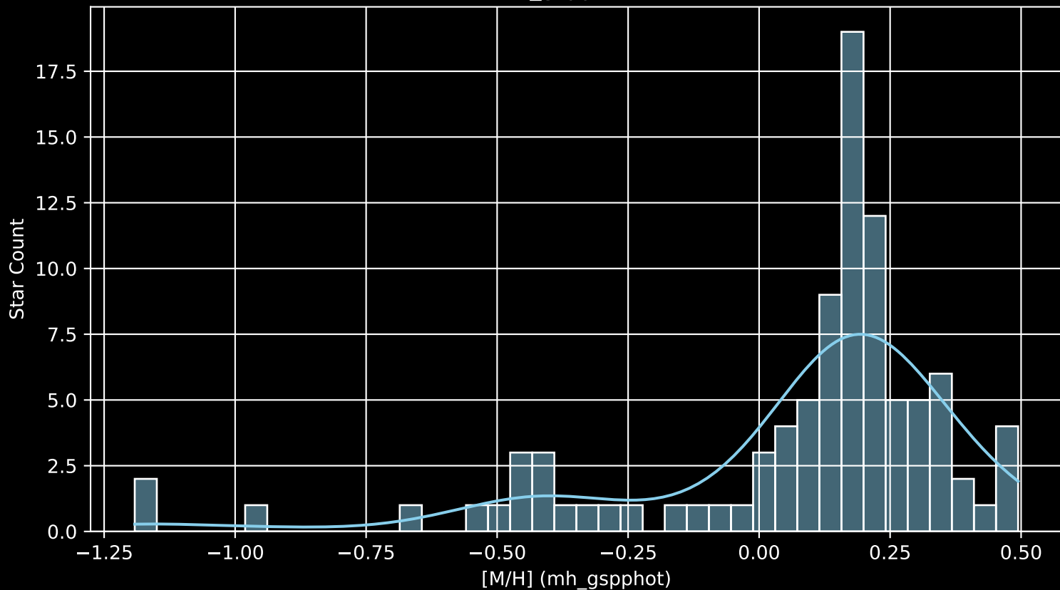
APOGEE DR17 Field: [LMC34 [M/H] (mh_gspphot) (n= 95)
